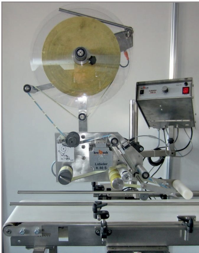
Labeler K80S, mounted on inlet-conveyor
