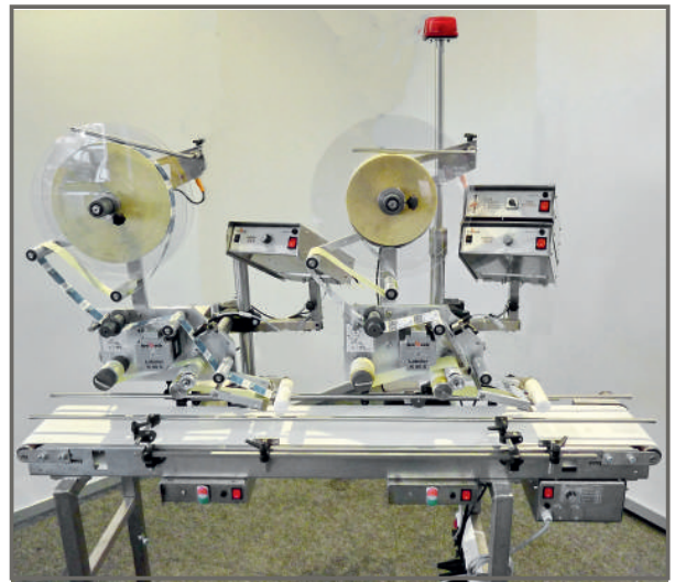
Twin version of K80S
